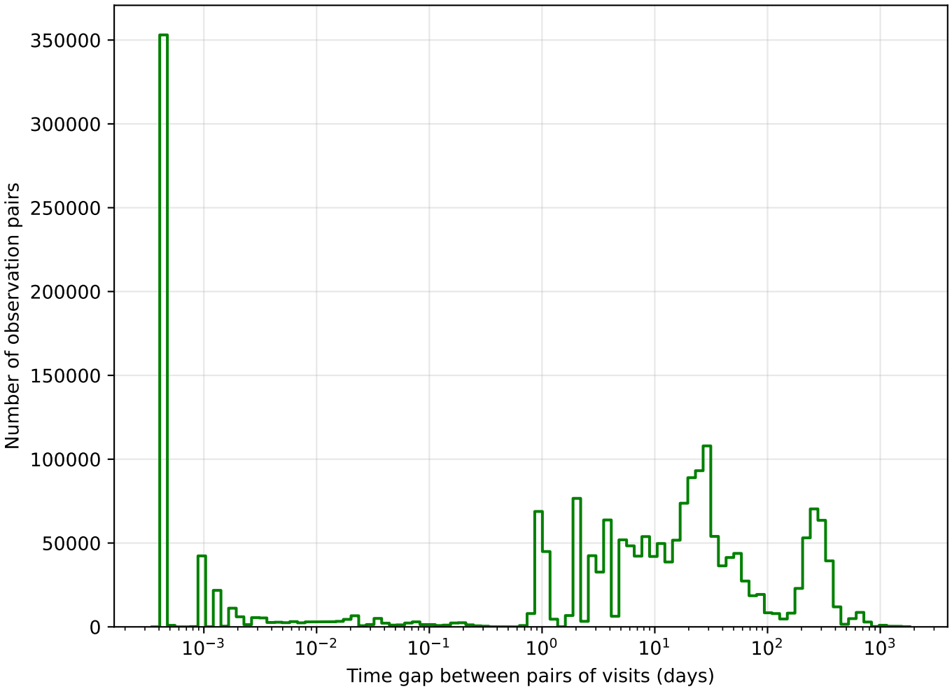
too_elab_r32_d3_griz_v3.4_10yrs g band: Tgaps observationStartMJD
