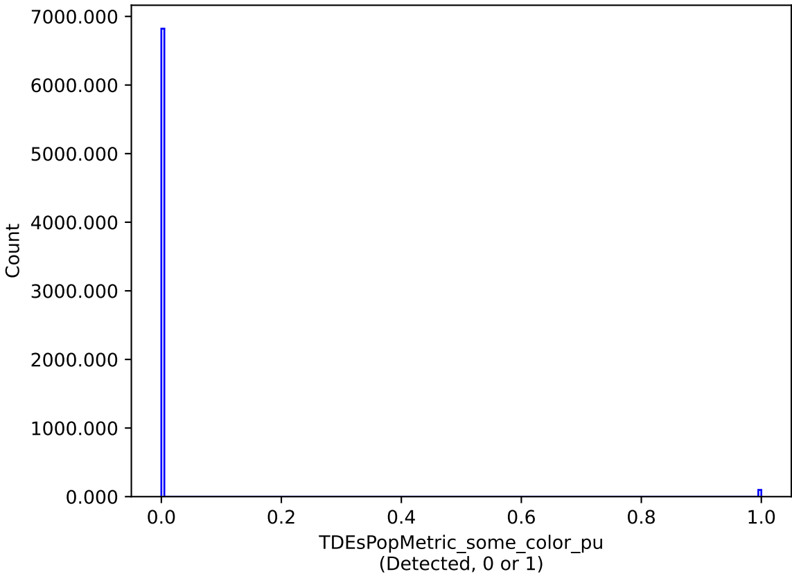
too_elab_r32_d3_griz_v3.4_10yrs : TDEsPopMetric_some_color_pu
