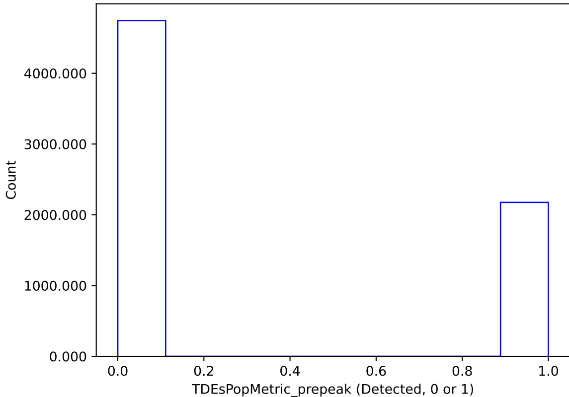
too_elab_r32_d3_griz_v3.4_10yrs : TDEsPopMetric_prepeak
