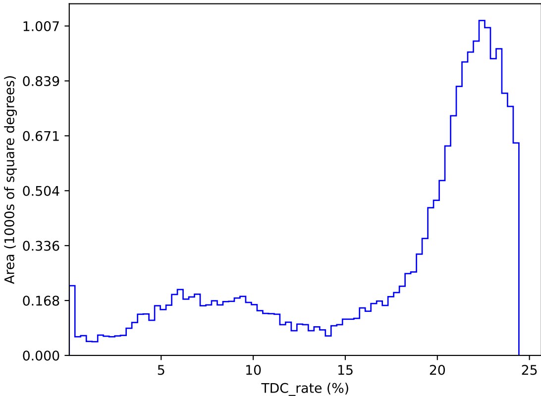
too_elab_r32_d3_griz_v3.4_10yrs : TDC_rate
