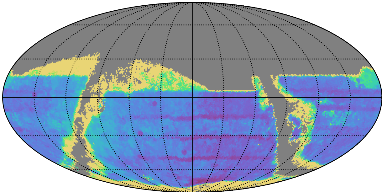
too_elab_r32_d3_griz_v3.4_10yrs : TDC_accuracy
