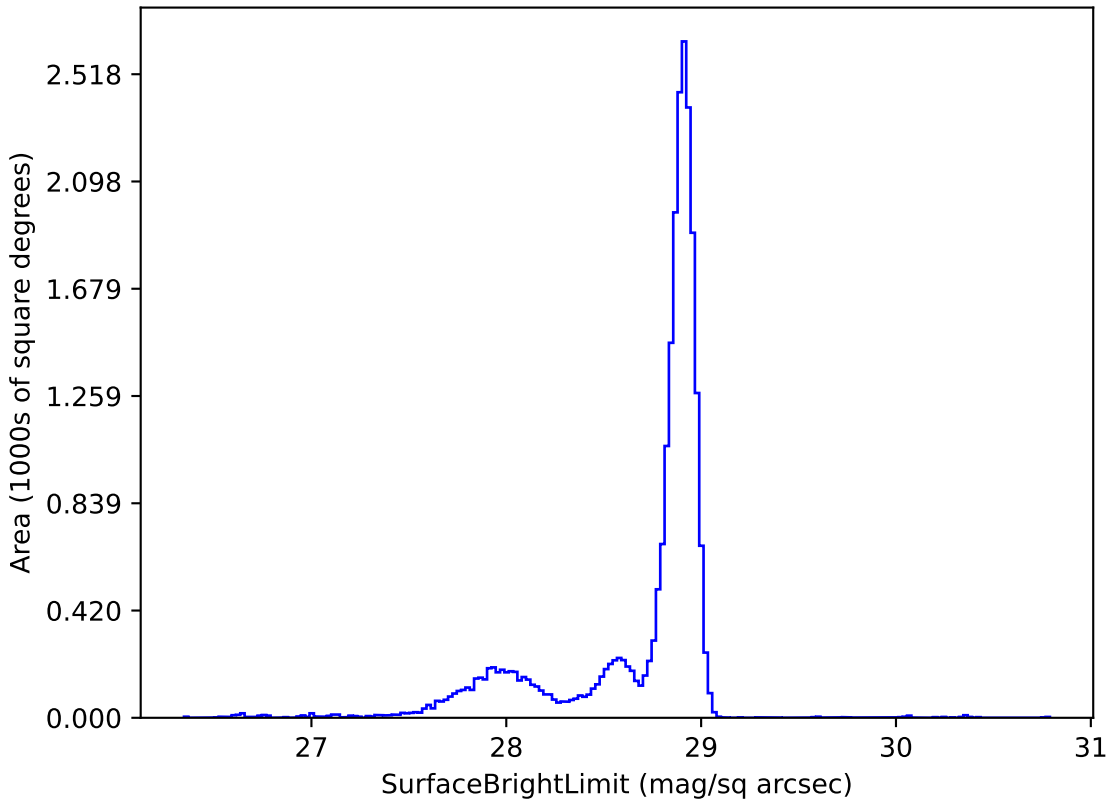
too_elab_r32_d3_griz_v3.4_10yrs u: SurfaceBrightLimit
