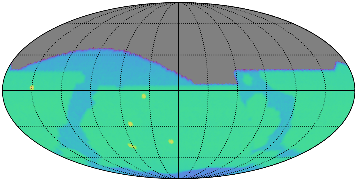
too_elab_r32_d3_griz_v3.4_10yrs i: SurfaceBrightLimit
