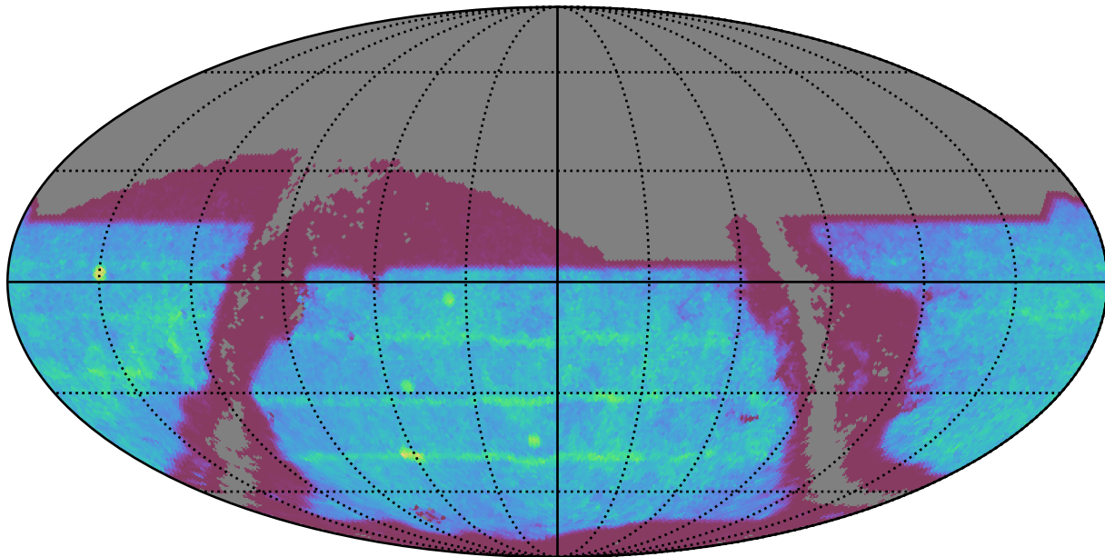
too_elab_r32_d3_griz_v3.4_10yrs : SNSLMetric
