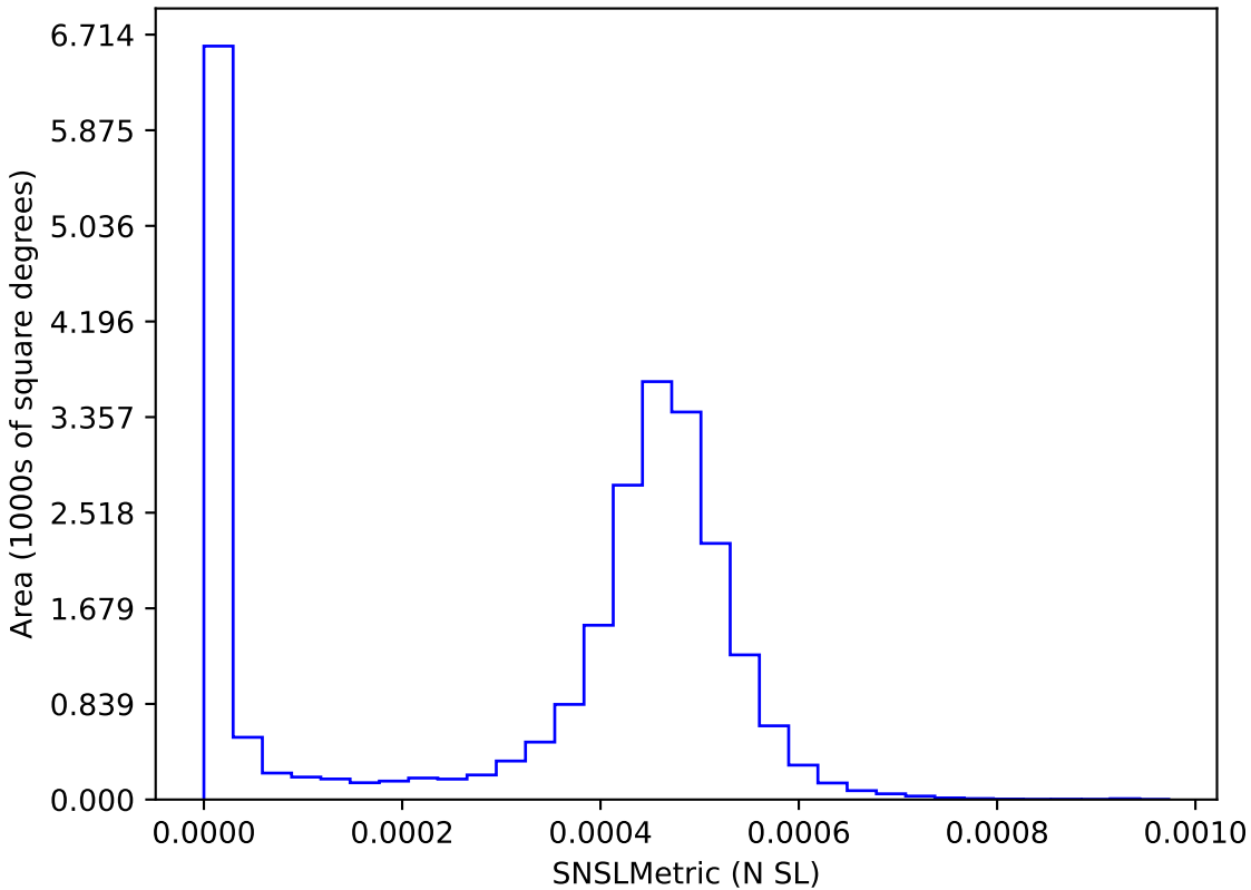
too_elab_r32_d3_griz_v3.4_10yrs : SNSLMetric
