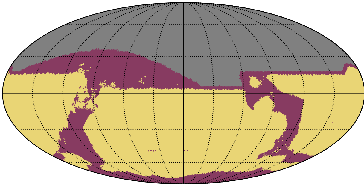
too_elab_r32_d3_griz_v3.4_10yrs : RapidRevisits
