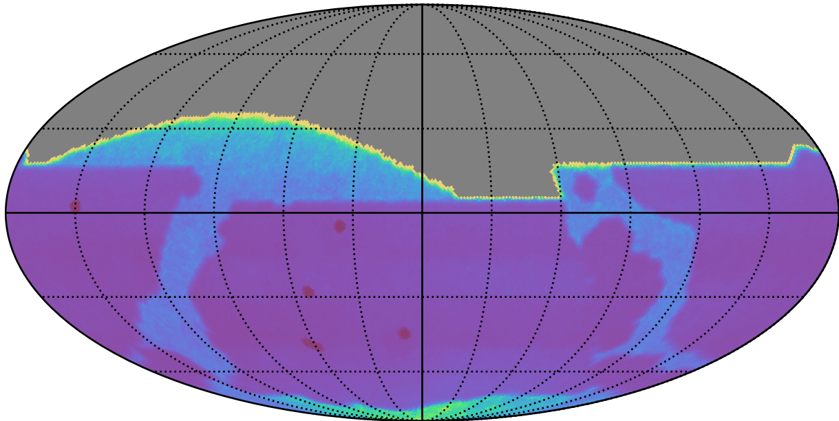
too_elab_r32_d3_griz_v3.4_10yrs : Proper Motion Uncert @ 20.5
