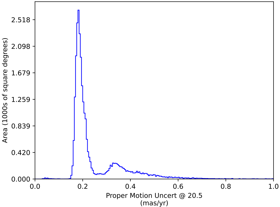
too_elab_r32_d3_griz_v3.4_10yrs : Proper Motion Uncert @ 20.5
