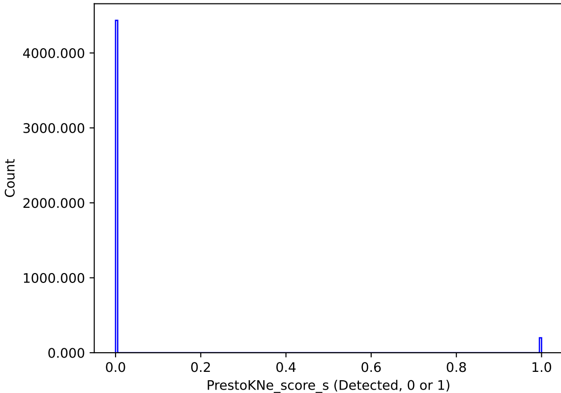
too_elab_r32_d3_griz_v3.4_10yrs : PrestoKNe_score_s
