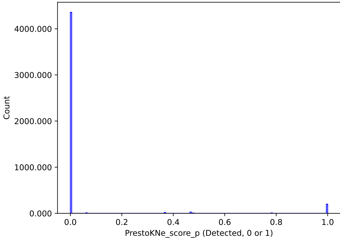
too_elab_r32_d3_griz_v3.4_10yrs : PrestoKNe_score_p
