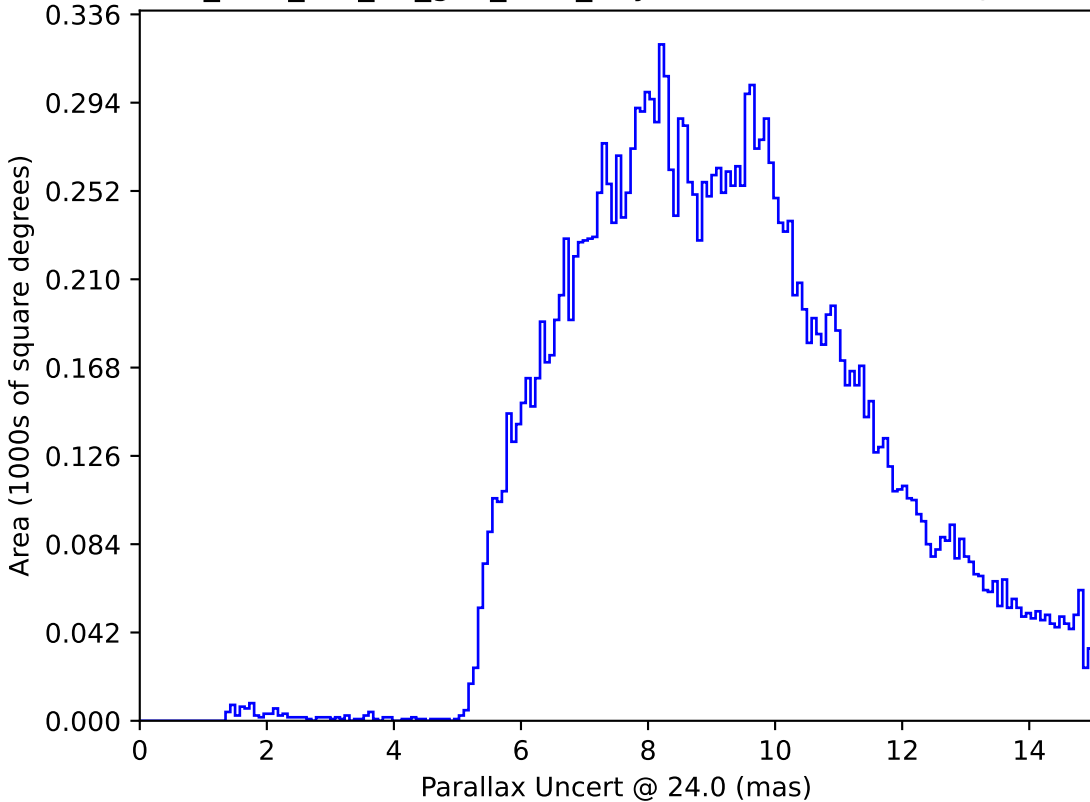
too_elab_r32_d3_griz_v3.4_10yrs : Parallax Uncert @ 24.0
