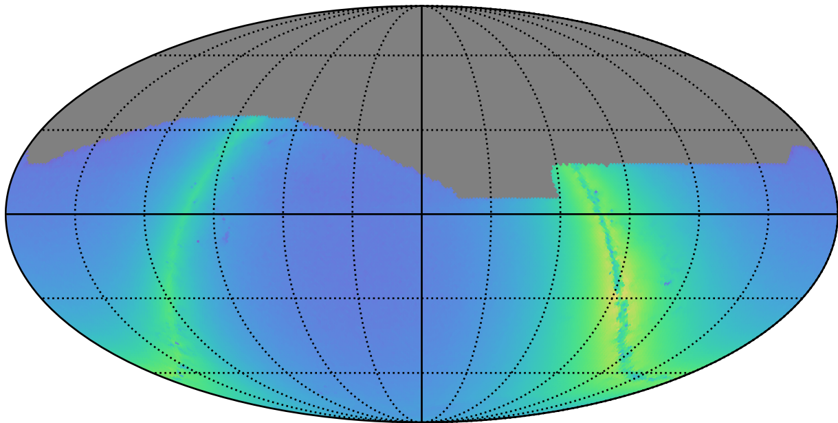
too_elab_r32_d3_griz_v3.4_10yrs i: Nstars_no_crowding
