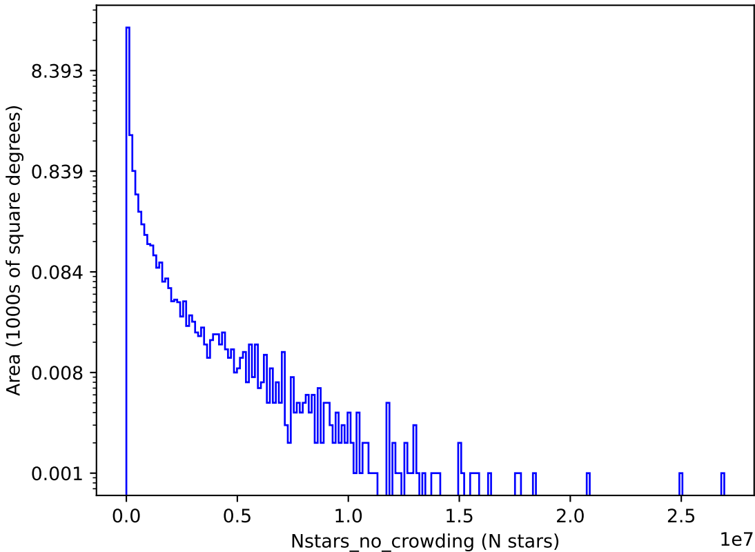
too_elab_r32_d3_griz_v3.4_10yrs i: Nstars_no_crowding
