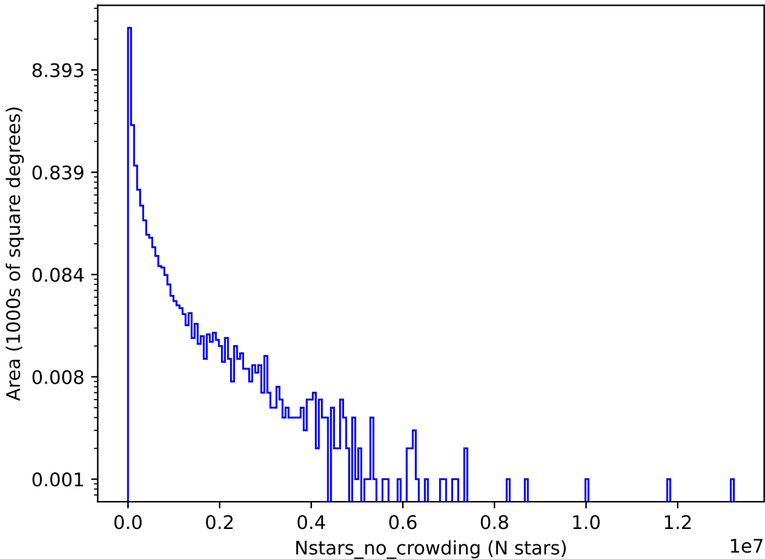
too_elab_r32_d3_griz_v3.4_10yrs g: Nstars_no_crowding
