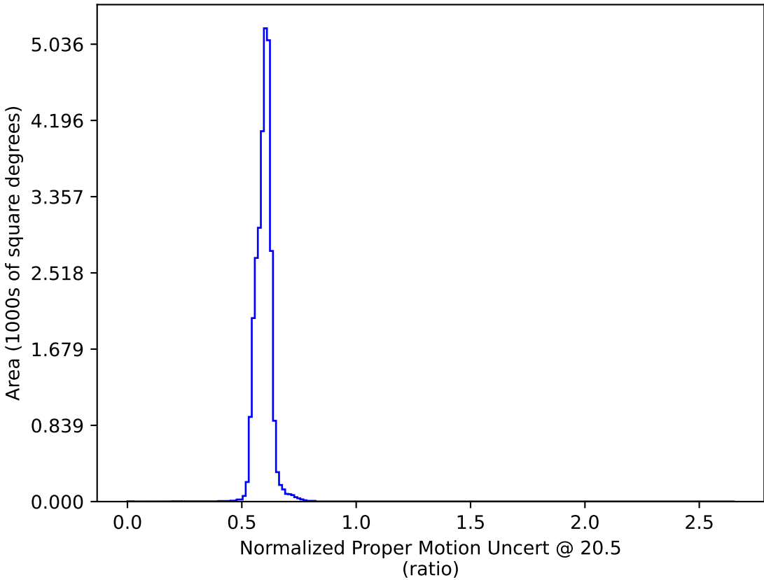
too_elab_r32_d3_griz_v3.4_10yrs : Normalized Proper Motion Uncert @ 20.5
