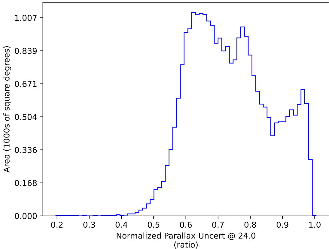
too_elab_r32_d3_griz_v3.4_10yrs : Normalized Parallax Uncert @ 24.0
