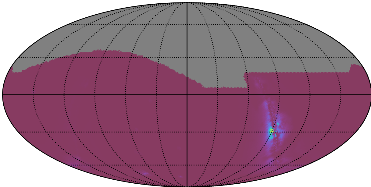
too_elab_r32_d3_griz_v3.4_10yrs : NlcPoints
