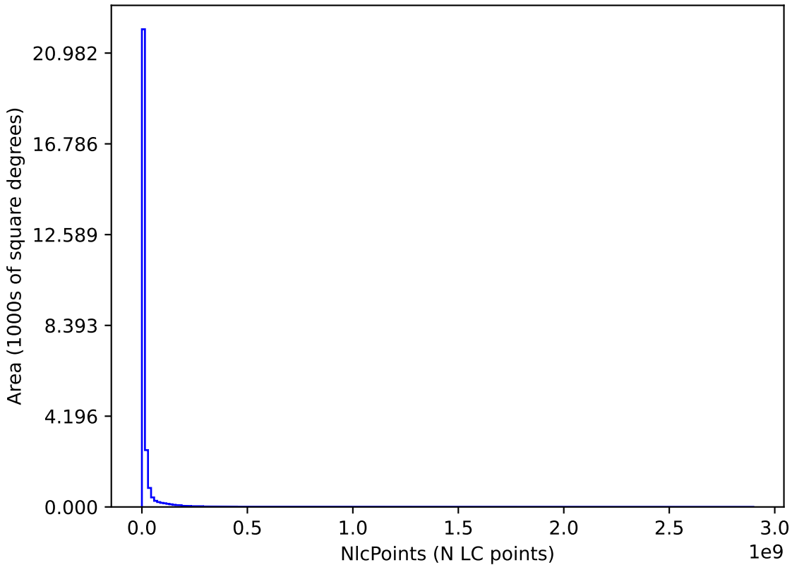
too_elab_r32_d3_griz_v3.4_10yrs : NlcPoints
