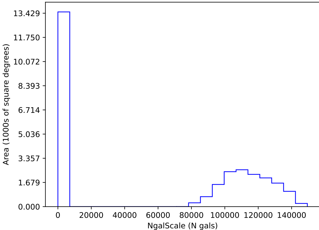
too_elab_r32_d3_griz_v3.4_10yrs i: NgalScale
