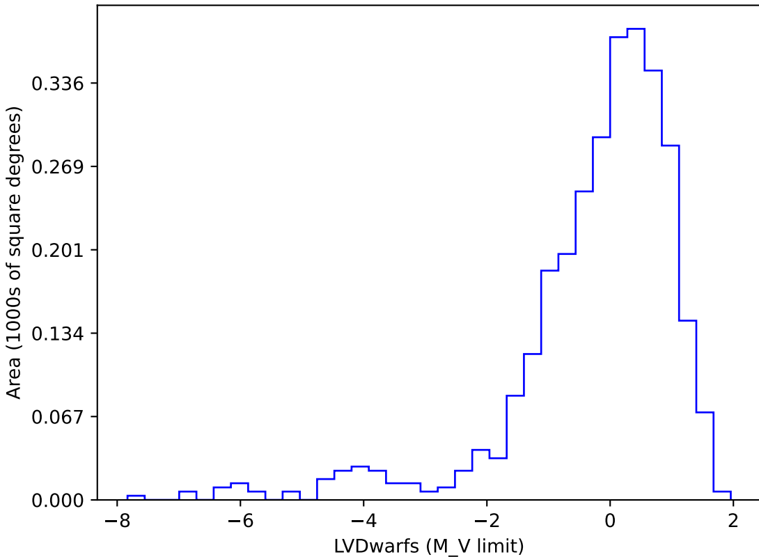
too_elab_r32_d3_griz_v3.4_10yrs gi SCP: LVDwarfs
