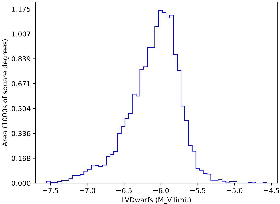
too_elab_r32_d3_griz_v3.4_10yrs gi: LVDwarfs
