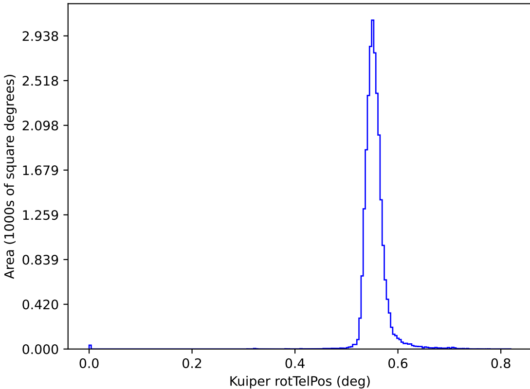
too_elab_r32_d3_griz_v3.4_10yrs y: Kuiper rotTelPos
