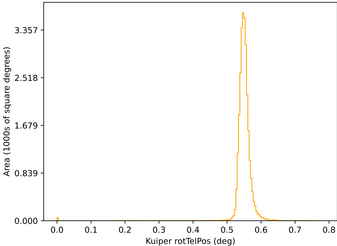
too_elab_r32_d3_griz_v3.4_10yrs r: Kuiper rotTelPos
