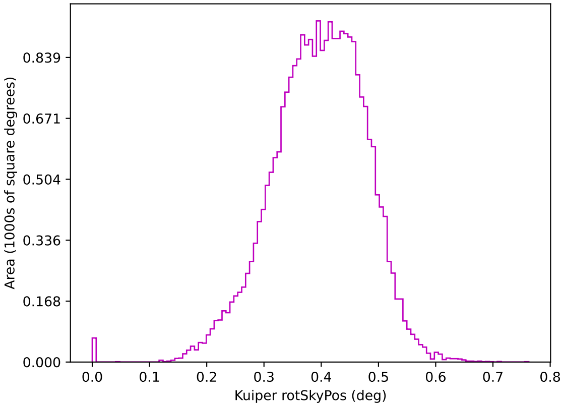
too_elab_r32_d3_griz_v3.4_10yrs z: Kuiper rotSkyPos
