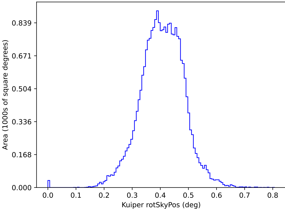
too_elab_r32_d3_griz_v3.4_10yrs y: Kuiper rotSkyPos
