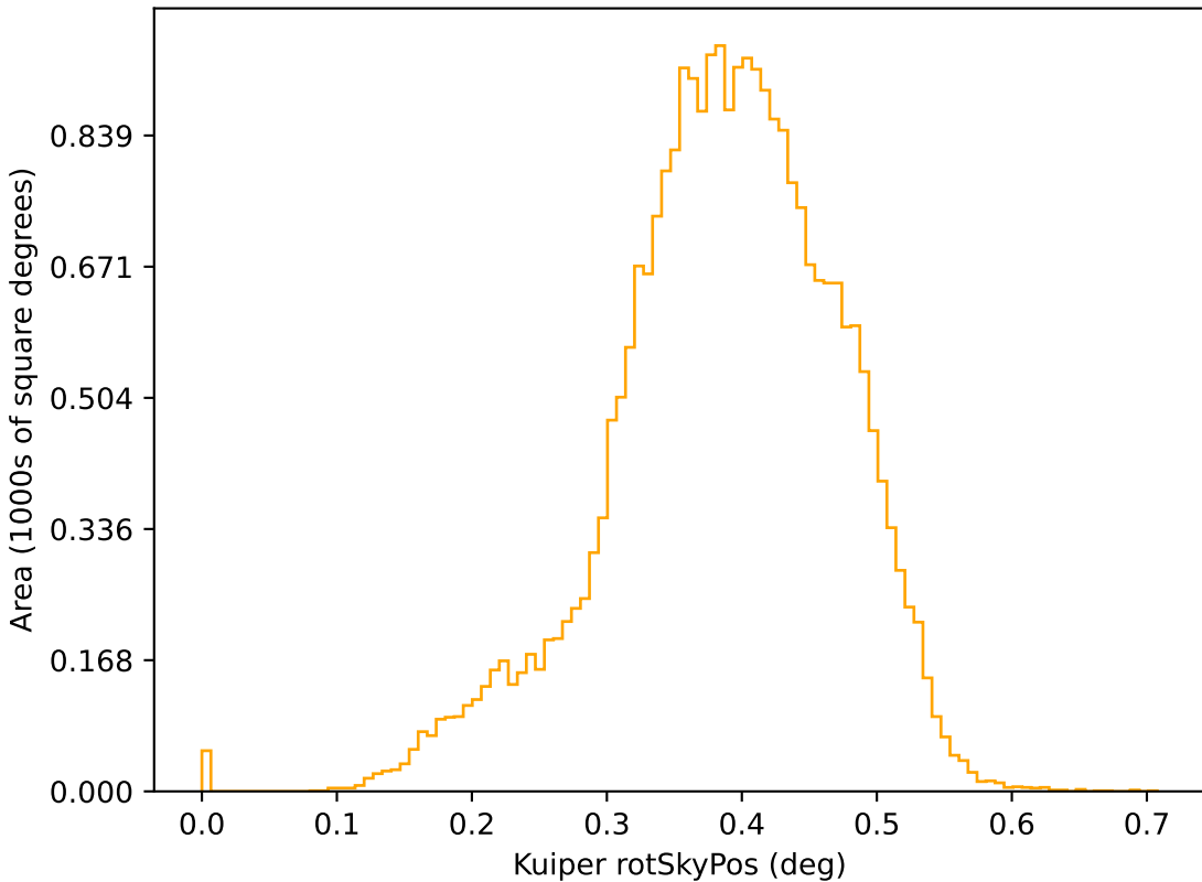
too_elab_r32_d3_griz_v3.4_10yrs r: Kuiper rotSkyPos
