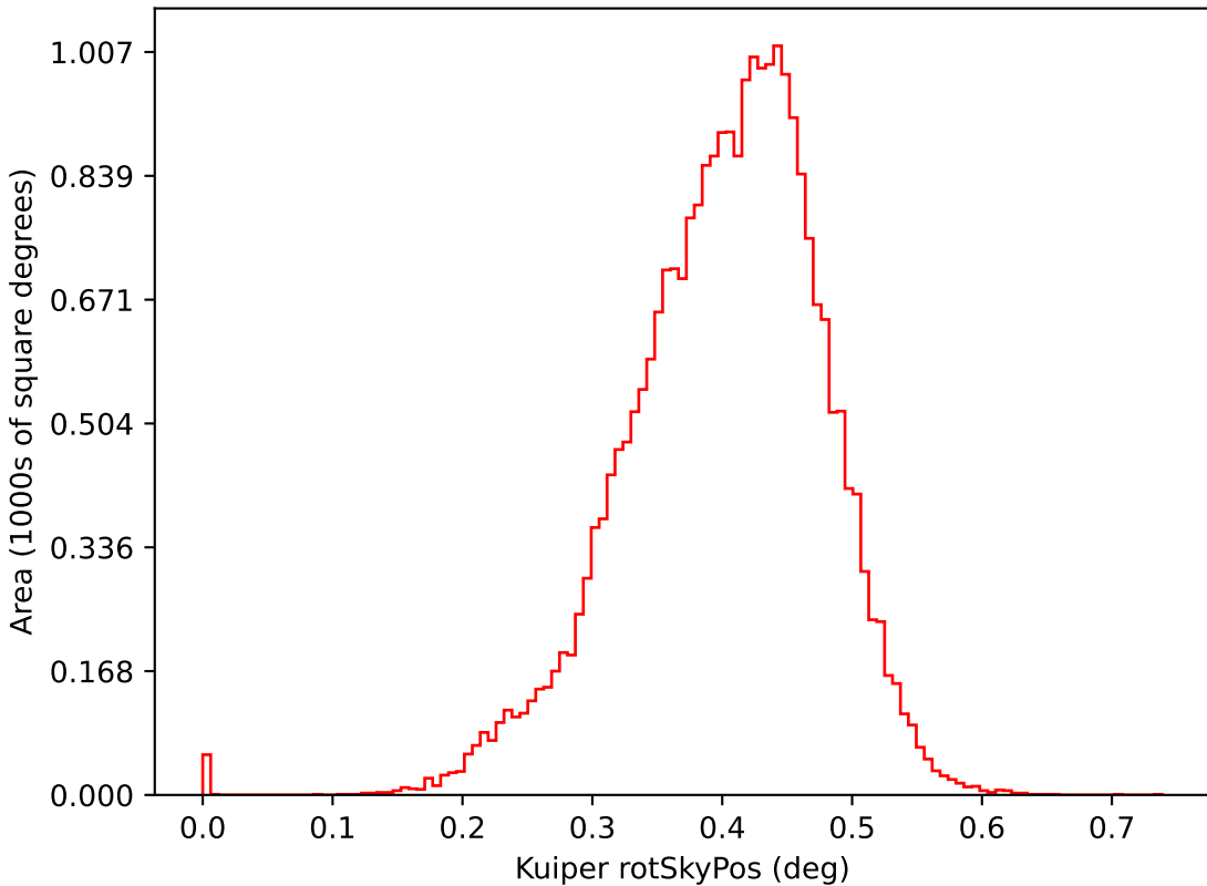
too_elab_r32_d3_griz_v3.4_10yrs i: Kuiper rotSkyPos
