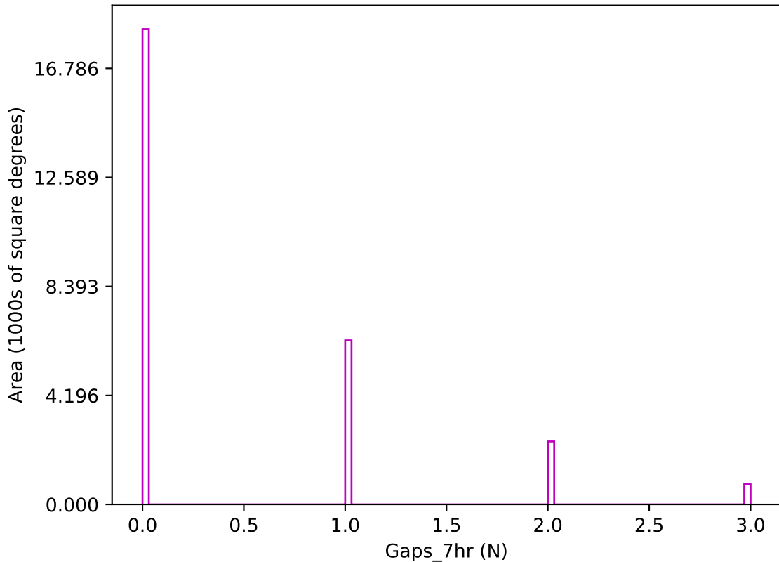
too_elab_r32_d3_griz_v3.4_10yrs z band: Gaps_7hr
