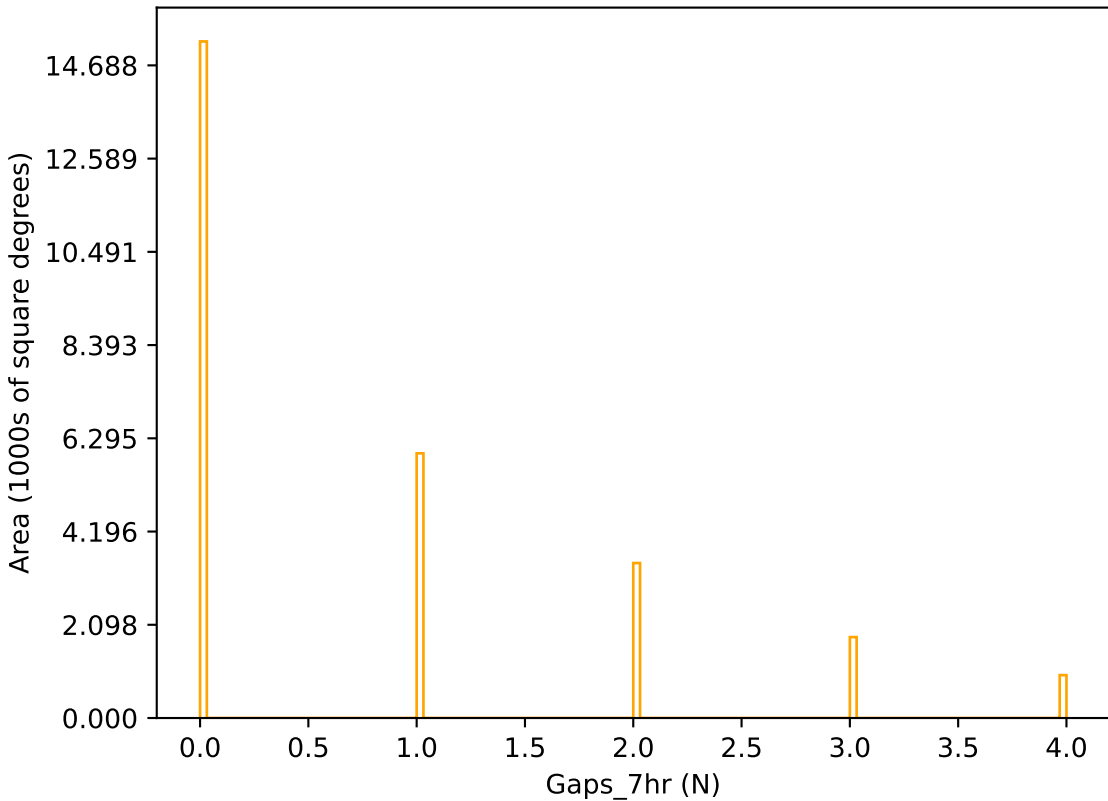
too_elab_r32_d3_griz_v3.4_10yrs r band: Gaps_7hr
