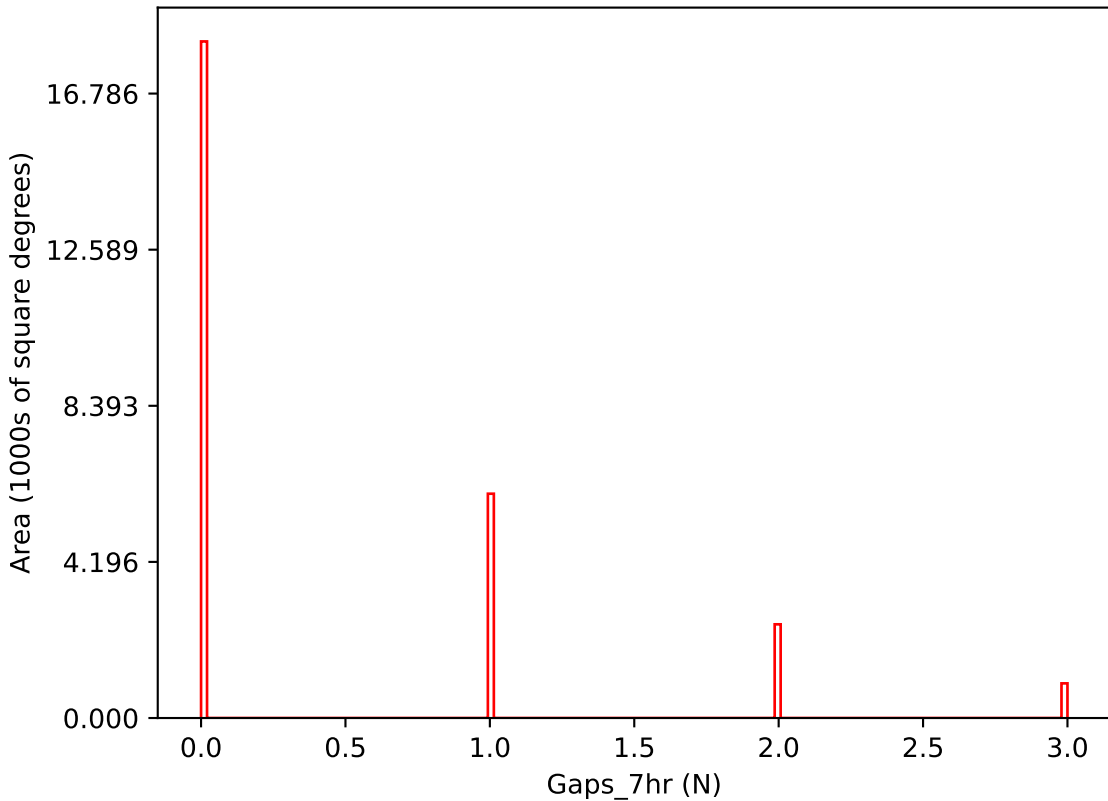
too_elab_r32_d3_griz_v3.4_10yrs i band: Gaps_7hr
