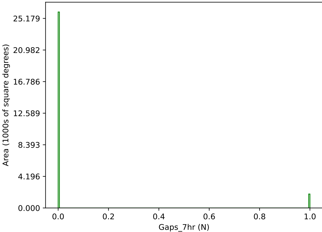
too_elab_r32_d3_griz_v3.4_10yrs g band: Gaps_7hr
