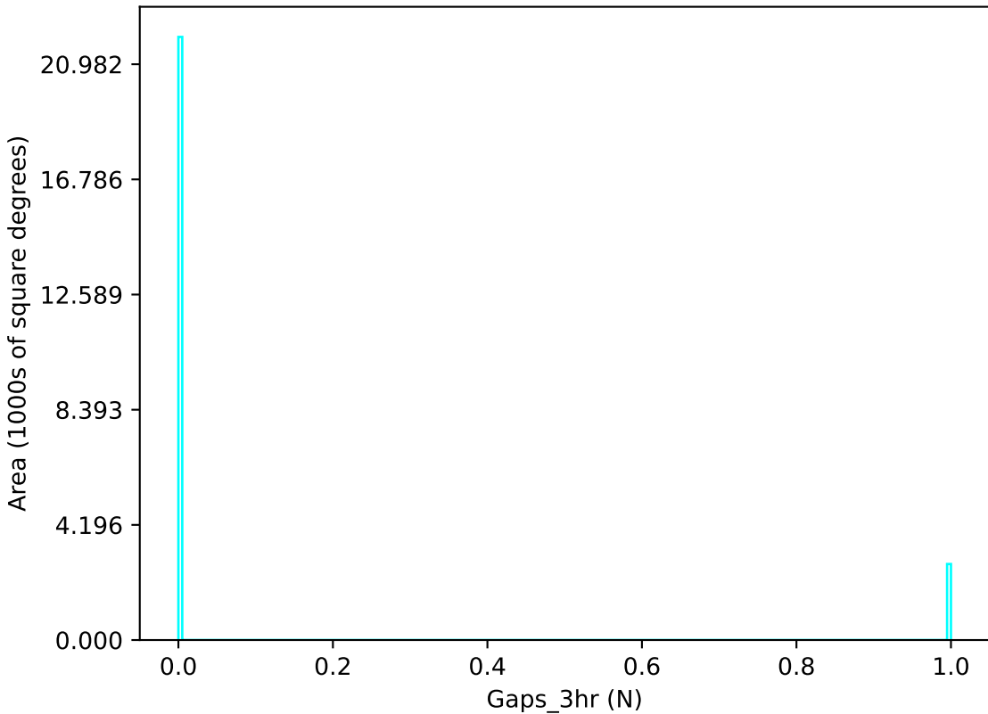
too_elab_r32_d3_griz_v3.4_10yrs u band: Gaps_3hr
