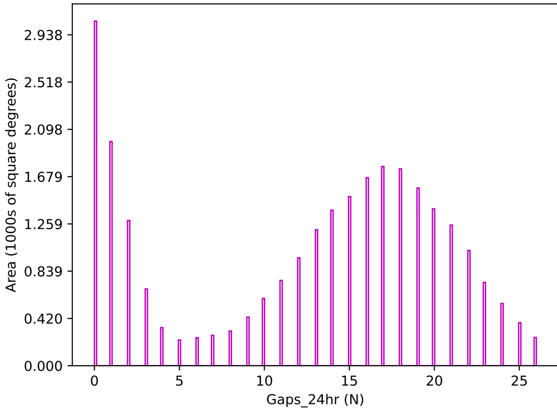
too_elab_r32_d3_griz_v3.4_10yrs z band: Gaps_24hr
