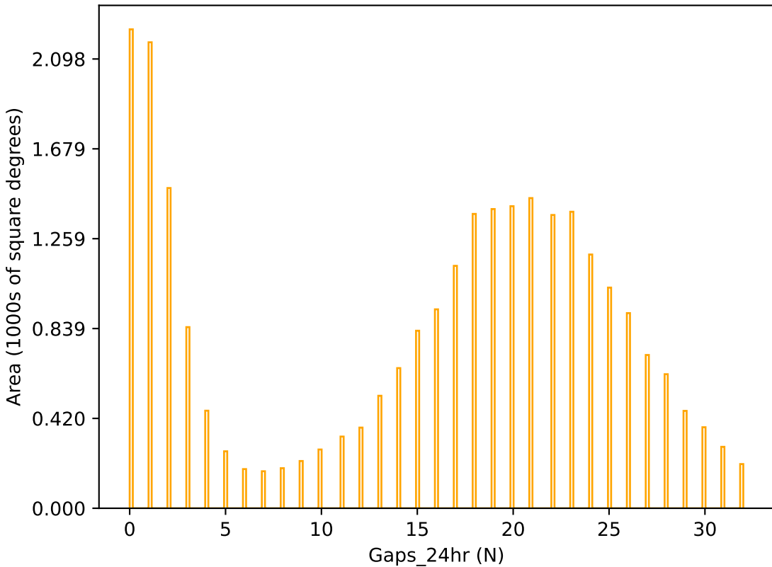
too_elab_r32_d3_griz_v3.4_10yrs r band: Gaps_24hr
