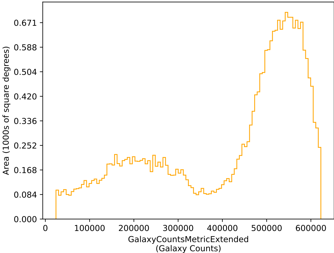
too_elab_r32_d3_griz_v3.4_10yrs r: GalaxyCountsMetricExtended
