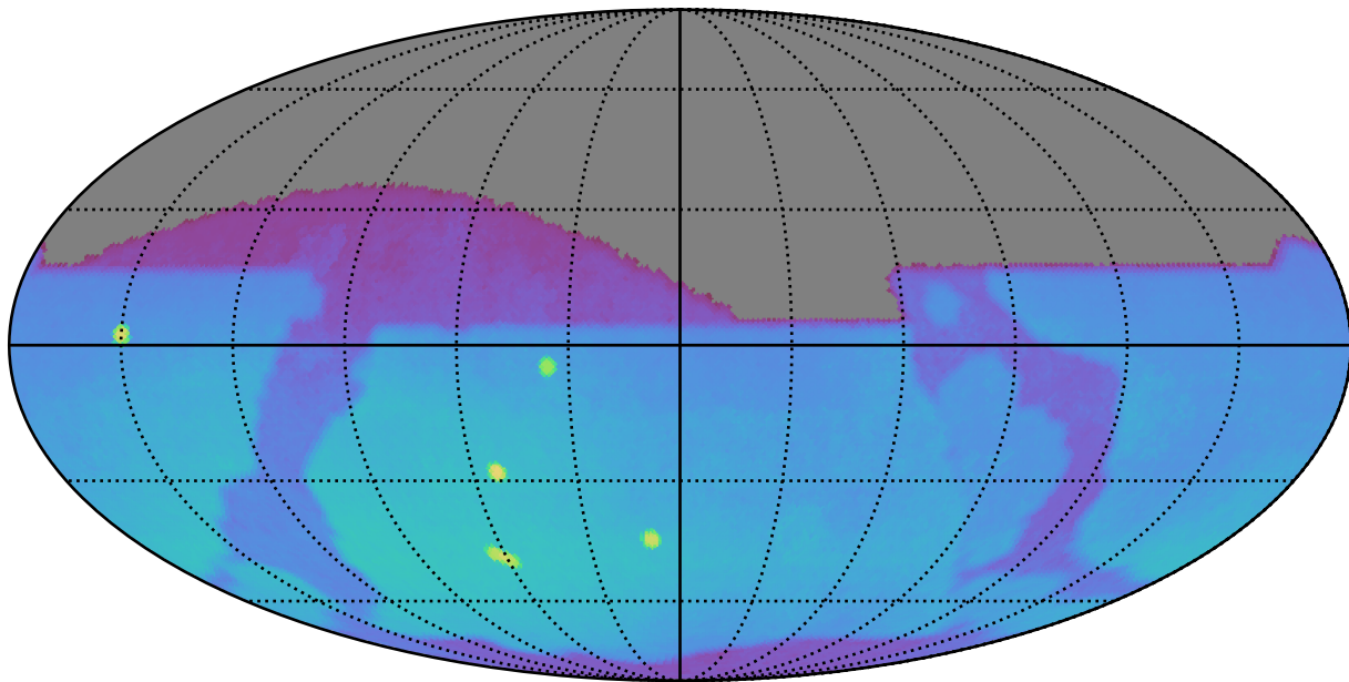
too_elab_r32_d3_griz_v3.4_10yrs : Brown Dwarf, L7
