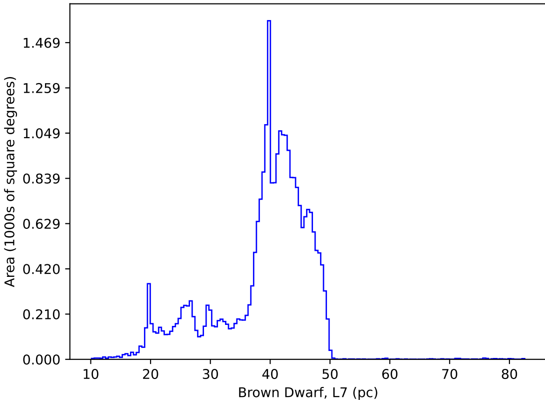
too_elab_r32_d3_griz_v3.4_10yrs : Brown Dwarf, L7
