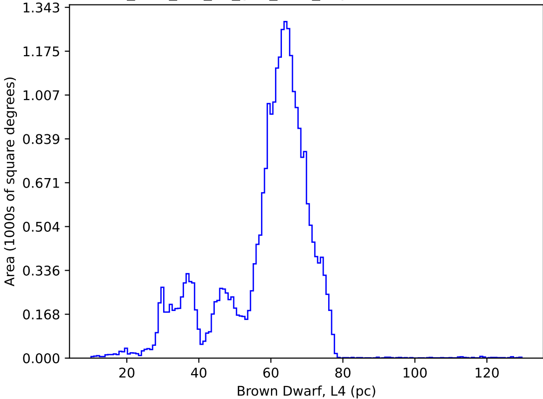
too_elab_r32_d3_griz_v3.4_10yrs : Brown Dwarf, L4
