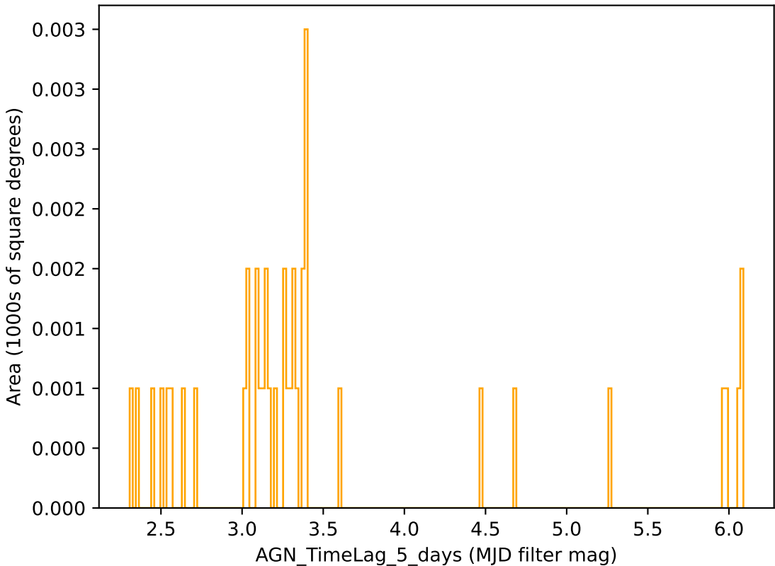
too_elab_r32_d3_griz_v3.4_10yrs r band: AGN_TimeLag_5_days
