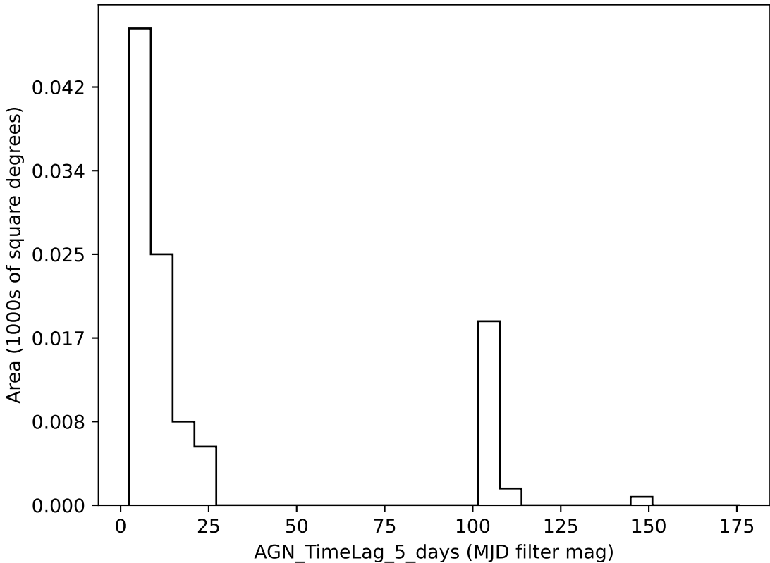
too_elab_r32_d3_griz_v3.4_10yrs all bands: AGN_TimeLag_5_days
