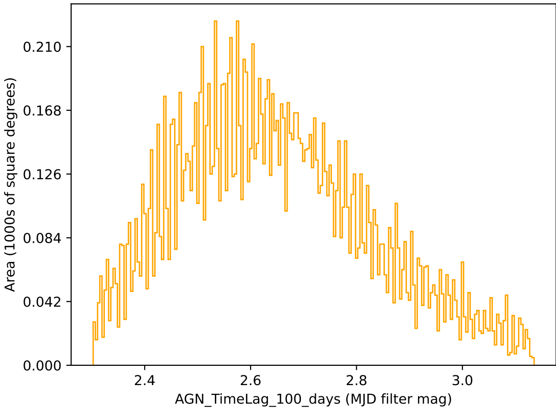
too_elab_r32_d3_griz_v3.4_10yrs r band: AGN_TimeLag_100_days
