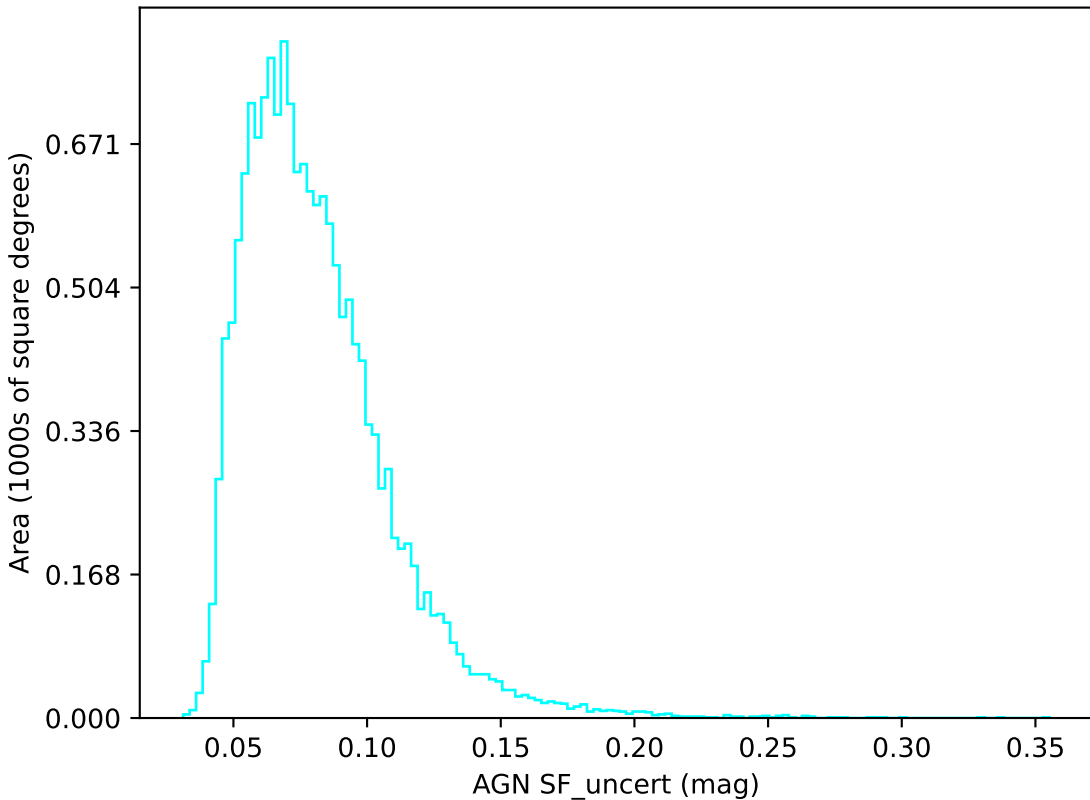
too_elab_r32_d3_griz_v3.4_10yrs u band: AGN SF_uncert
