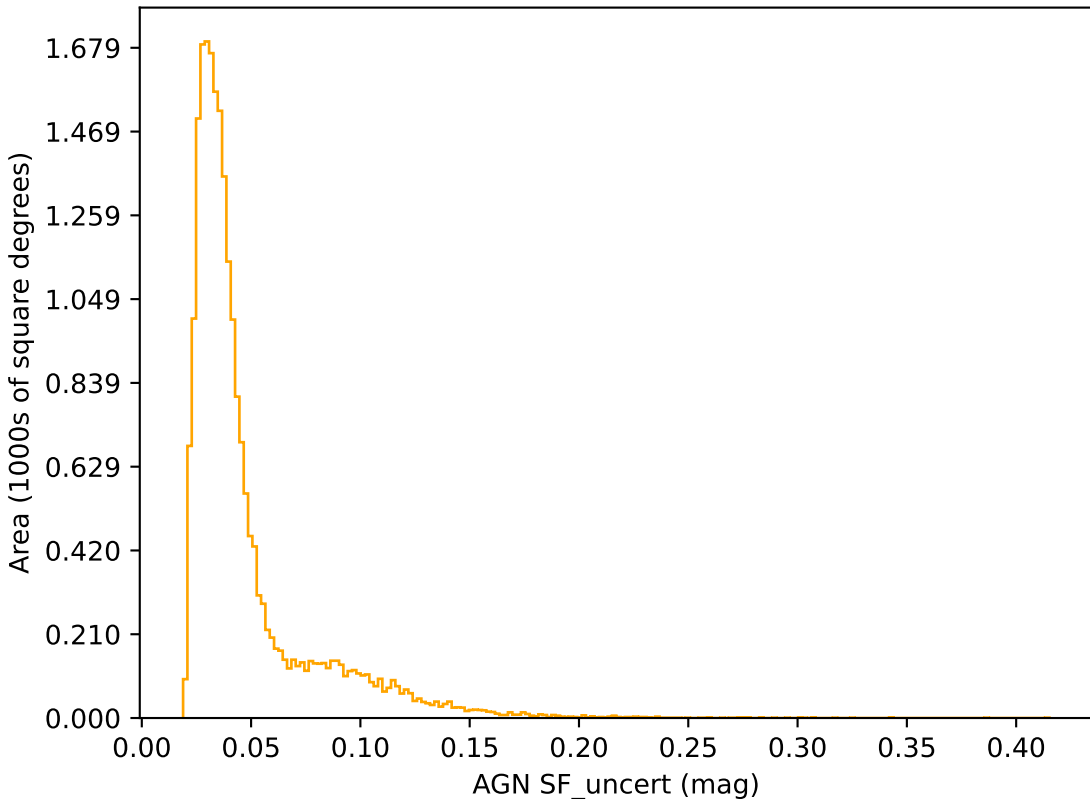
too_elab_r32_d3_griz_v3.4_10yrs r band: AGN SF_uncert
