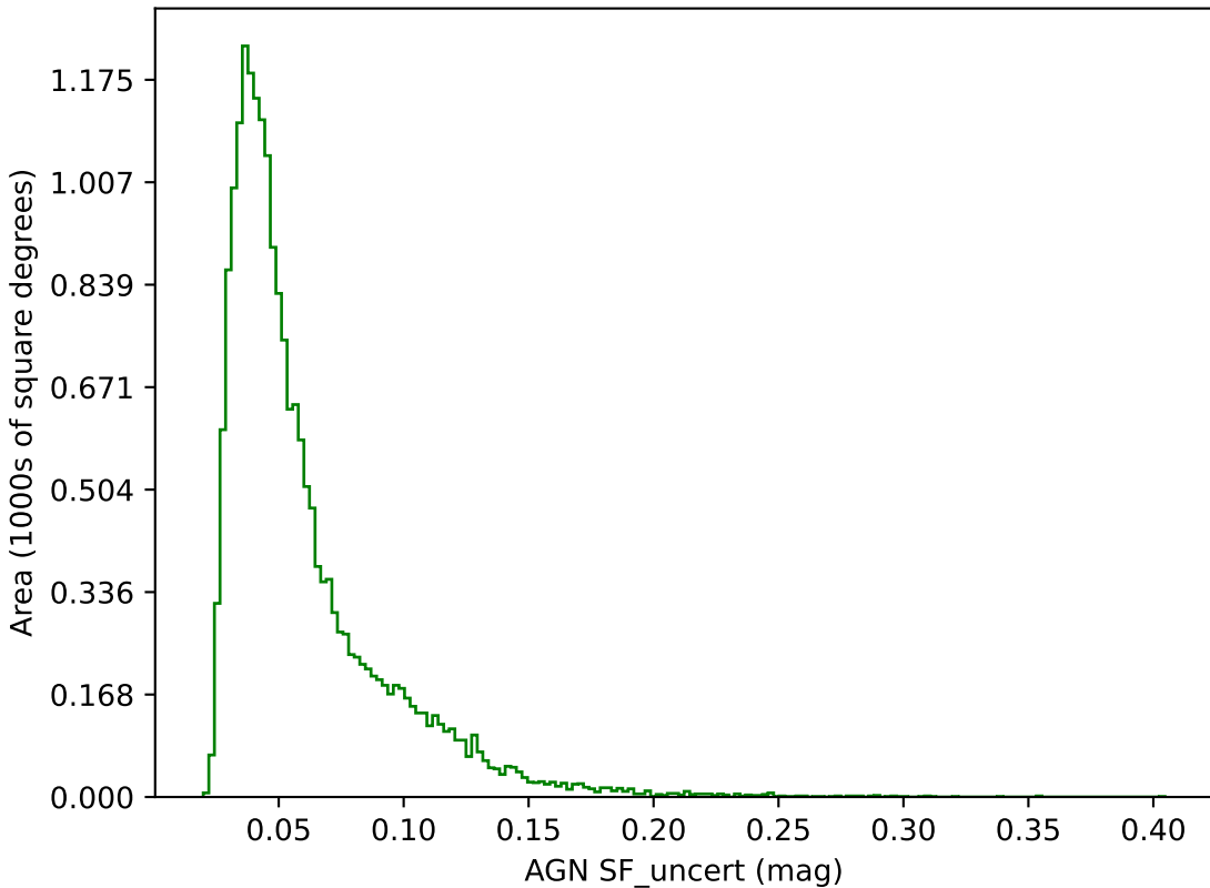
too_elab_r32_d3_griz_v3.4_10yrs g band: AGN SF_uncert
