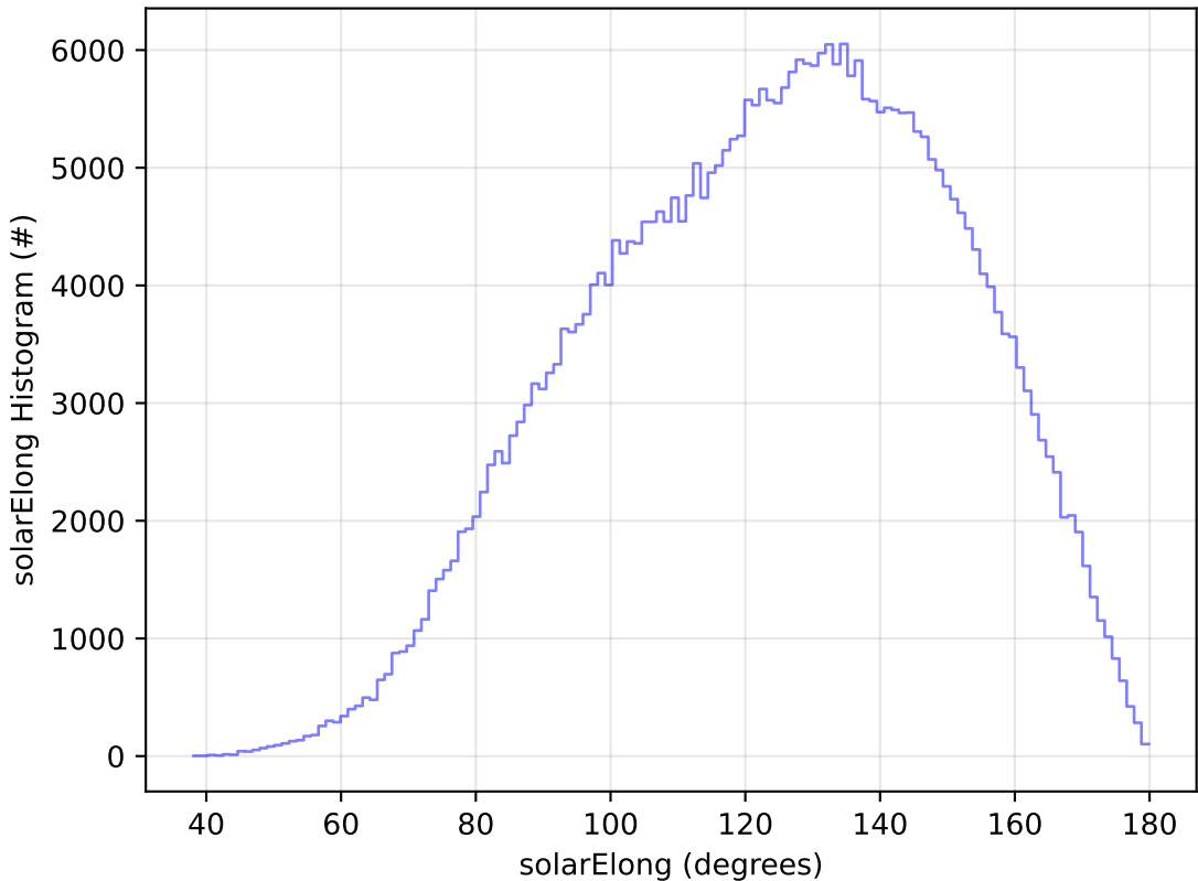
too_elab_r32_d3_griz_v3.4_10yrs WFD y band: solarElong Histogram
