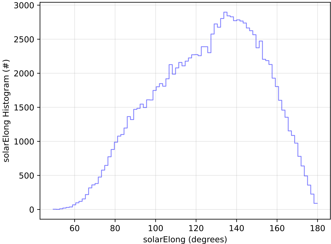
too_elab_r32_d3_griz_v3.4_10yrs WFD u band: solarElong Histogram
